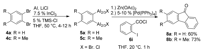
Scheme 3. Preparation of 1,2-dimetallic species 5a , 5c and subsequent acylation/cross-coupling sequence affording 9 H -fluorenone derivatives 8a , 8b .
