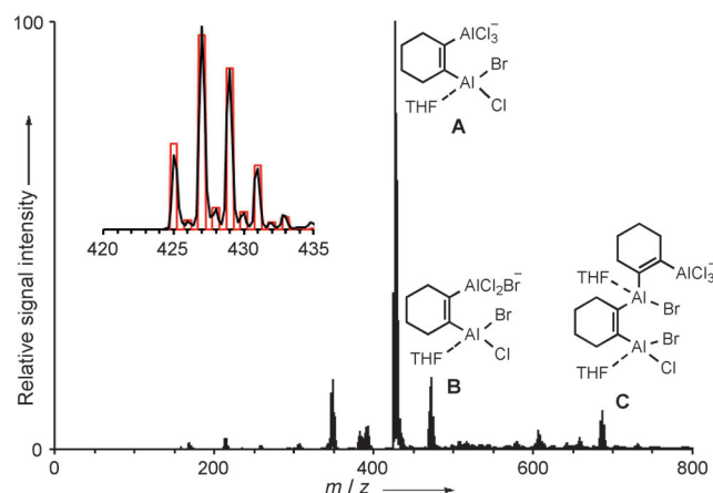
Figure 1. Negative-ion-mode ESI mass spectrum of a circa 10 mM solution of the products formed by reaction of 1 with Al powder in the presence of LiCl and InCl 3 in THF ( m/z ratios of the most abundant isotopologues: A : 427 [C 10 H 16 Al 2 BrCl 4 O] – ; B : 473 [C 10 H 16 Al 2 Br 2 Cl 3 O] – ; C : 687 [C 20 H 32 Al 3 Br 2 Cl 4 O 2 ] – ). Inset: measured (line, black) and simulated isotope pattern (bars, red) of A .
