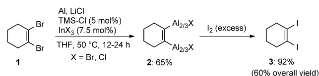
Scheme 1. Preparation of the dialuminum reagent 2 . [21] THF = tetrahydrofuran, TMS = trimethylsilyl.
