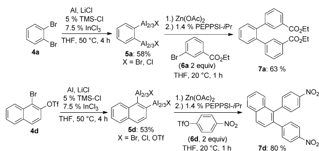
Scheme 2. Preparation of 1,2-dimetallic reagents 5a and 5d and subsequent cross-coupling reactions.
